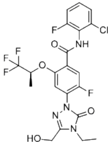
PC-3616101, DMSO-d6
